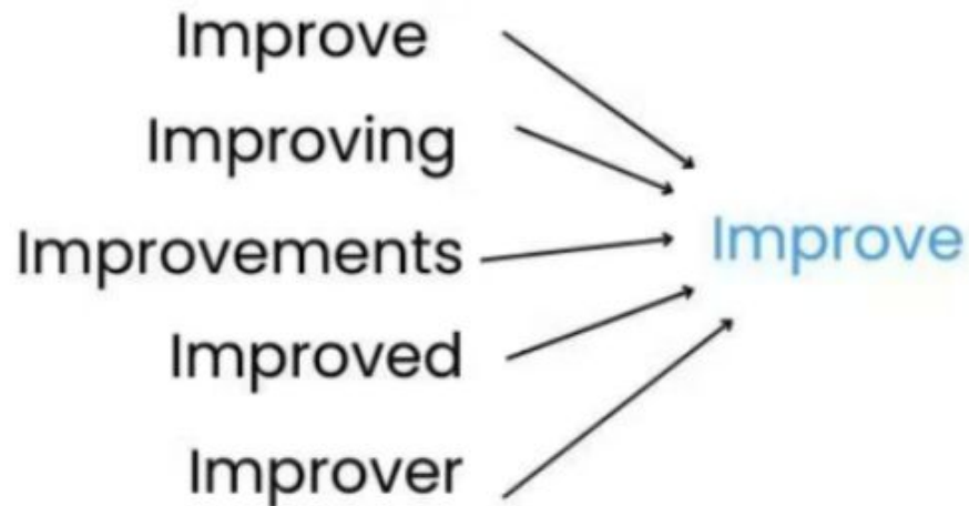
Lemmatization
